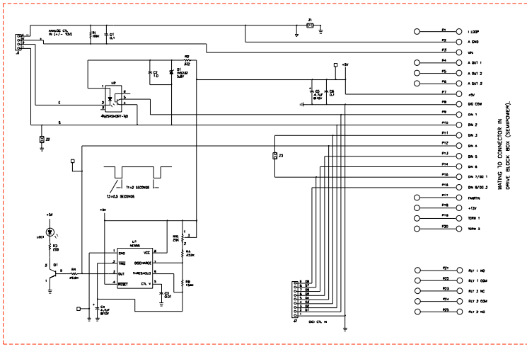
SCHEMATIC FOR DRIVE BOARD
