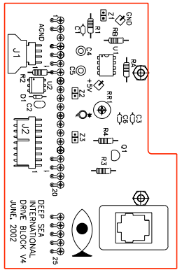
DRIVE PC BOARD COMPONENT LAYOUT
